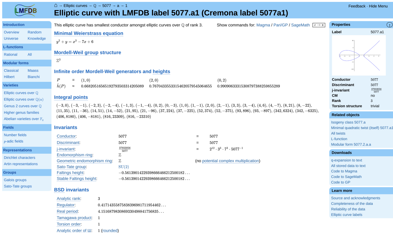
Figure 2: The homepage of the elliptic curve 5077.a1.
