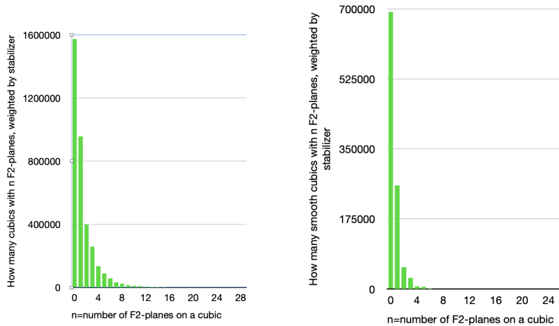
FIGURE 6. Stacky counts of the number of cubics containing n planes. A plot restricting to smooth cubics is given on the right.
