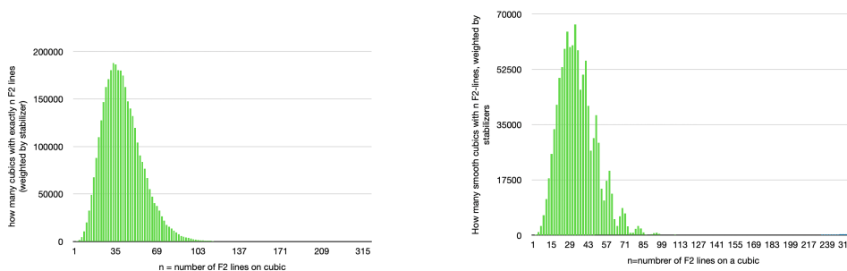
FIGURE 5. Stacky counts of the number of cubics containing n lines. A plot restricting to smooth cubics is given on the right.
